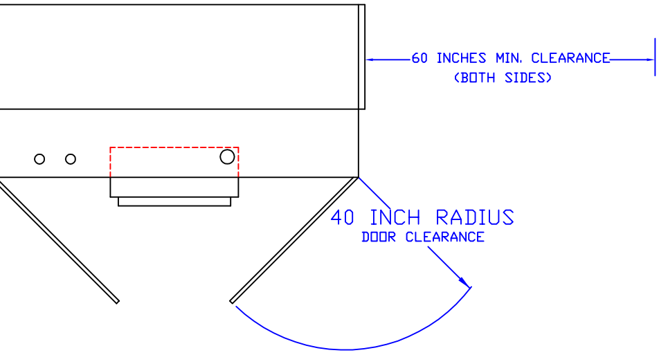
TOP VIEW OF CONTROL CABINET
