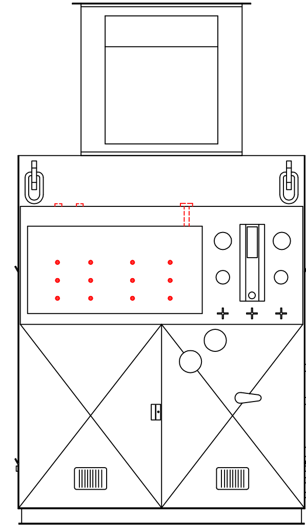
FRONT VIEW
